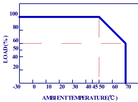
■Derating Curve
