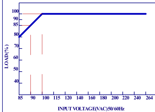
■Output load derating curve
